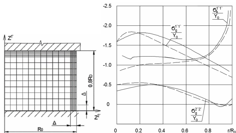
Fig. 2. The design scheme of the cylindrical workpiece and the graph of the distribution of axial and tangential stresses
