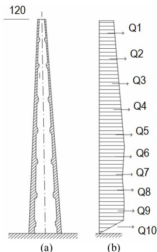
Fig. 3. General view of the pipe (a) and the diagram of the distribution of wind pressure (b)
