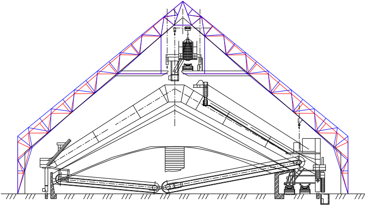
Fig. 5.1. The optimum design decision by the criterion of minimum structural weight when lower chord of the lattice rafter is straight-line.
