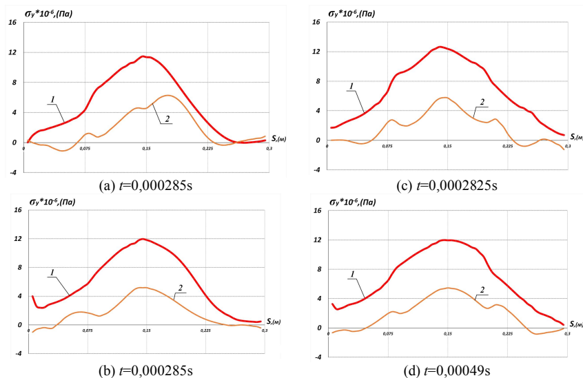
Fig. 3. Maximal stress \sigma_y of the shell bearing layers (1 – of the internal layer, 2 – of the external layer) provided the generatrix length of 295 mm and different taper angle values: (a) at E_{1,3}/E_T=500 and \alpha=10^\circ ; (b) at E_{1,3}/E_T=50 and \alpha=10^\circ ; (c) at E_{1,3}/E_T=500 and \alpha=20^\circ ; (d) at E_{1,3}/E_T=50 and \alpha=20^\circ
