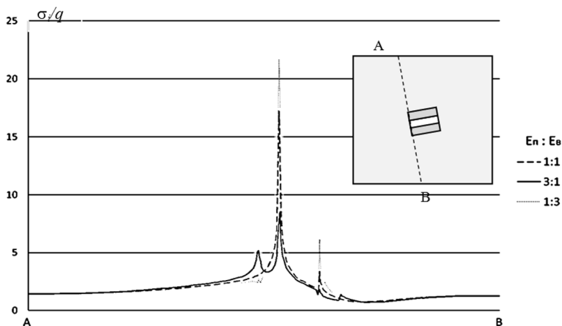
Fig. 10. Distribution of \sigma_z/q in section A-B at 60^\circ
