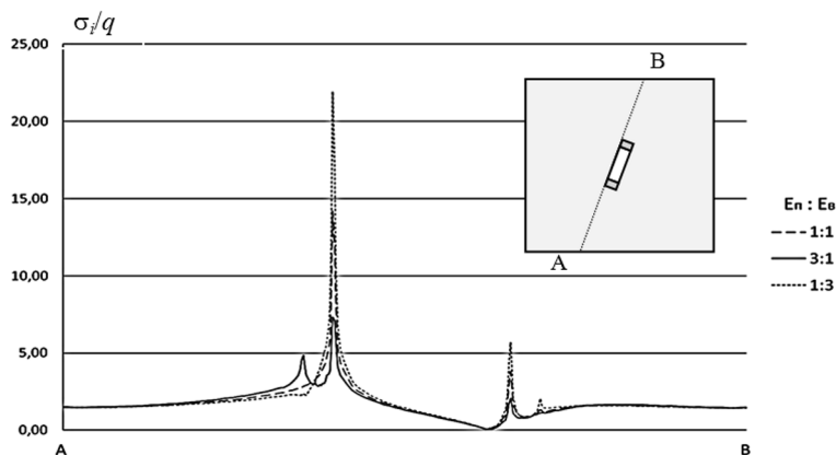
Fig. 3. Distribution of \sigma_i/q in section A–B at 30°
