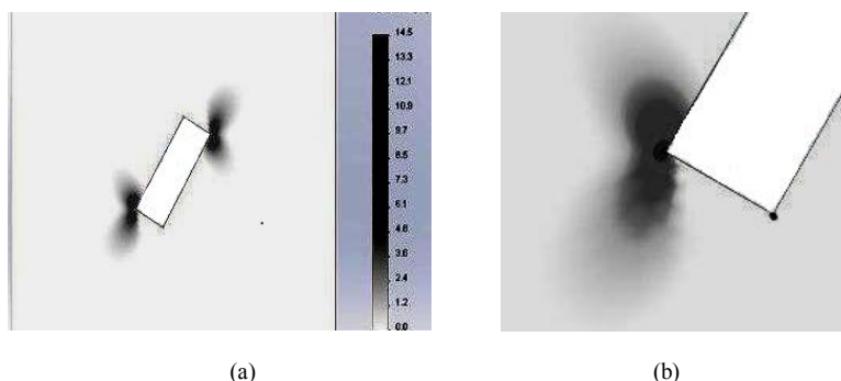
Fig. 2. Distribution of the relative stress intensity \sigma_i/q for the case shown in Fig. 1 (c):
