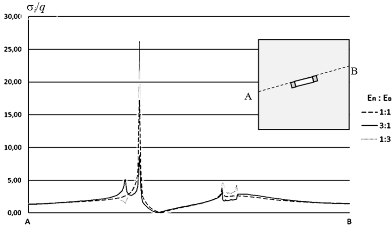
Fig. 7. Distribution of \sigma_z/q in section A-B at 60^\circ
