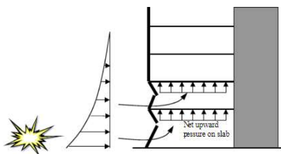
Fig. 13. Lifting of floor slabs by an explosive wave
