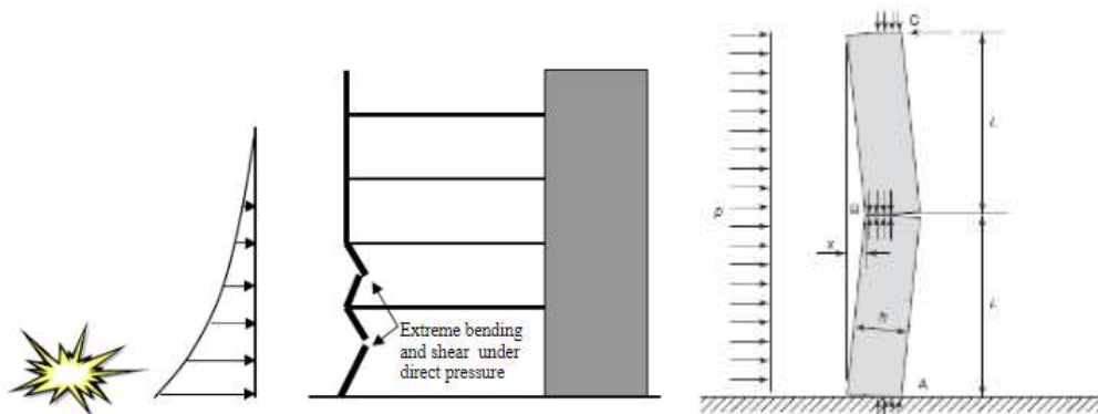
Fig. 12. Direct quasi-static loading of columns and walls by an explosive wave
