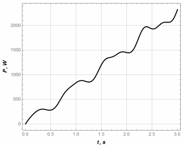
Fig. 9. Plot of consumed power of the belt conveyor drive mechanism
