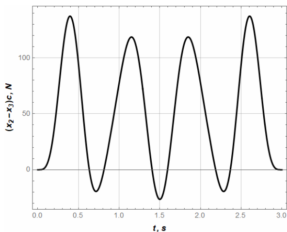
Fig. 7. Plot of the elastic force in the belt between the second and third masses
