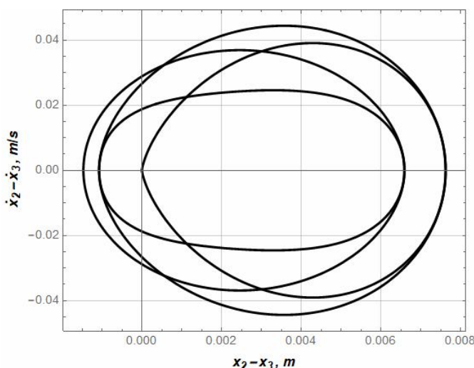
Fig. 5. Phase portrait of oscillations of the third mass relative to the second mass
