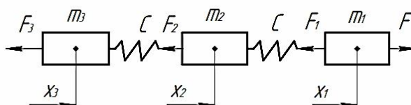
Fig. 1. A dynamic model of the belt conveyor
