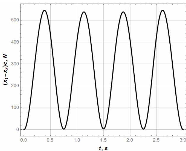
Fig. 6. Plot of the elastic force in the belt between the first and second masses
