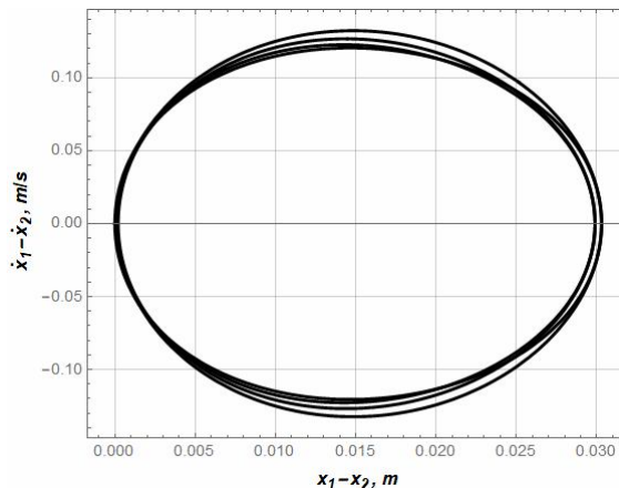
Fig. 4. Phase portrait of the oscillations of the second mass relative to the first one
