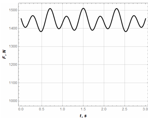
Fig. 8. Plot of the driving force of the belt conveyor drive mechanism
