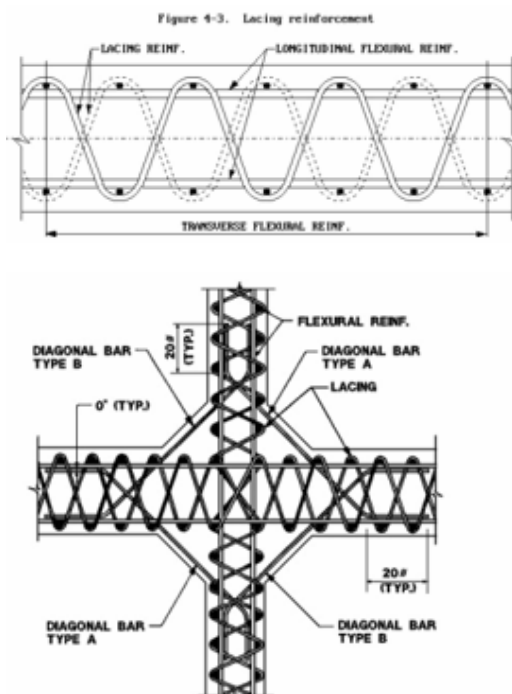
Figure 4-56. Typical detail at intersection of two continuous laced walls
