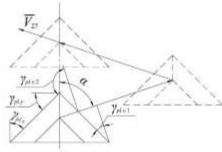
Fig. 6. Plan of movement of a spatially oriented knife at an angle \alpha > 45^\circ
