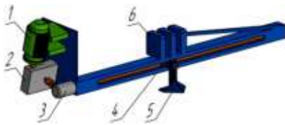
Fig. 12. 3D model of the construction of equipment for cutting soils with a spatially oriented knife
