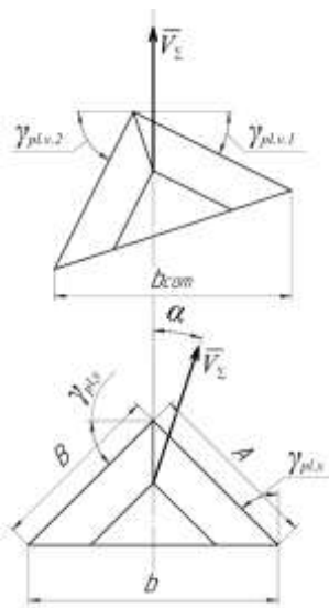
Fig. 7. Parameterization of spatial oriented knife when \gamma_{pl,y} > \alpha < \gamma_{pl,x}
