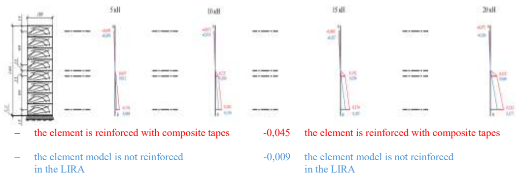
Fig. 16. Maximum longitudinal stresses in the wood of the investigated sections of the experimental specimen and the experimental specimen model in the LIRA software reinforced with composite strips, at load values of 5, 10, 15, and 20 kN, applied along a single load axis
