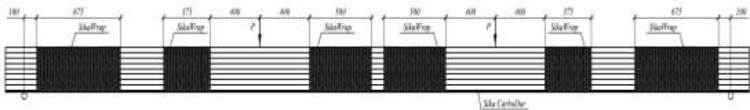
Fig. 22. Reinforcement scheme of zones of maximum stress concentration in glued laminated timber beams strengthened with composite strips according to Variant №1
