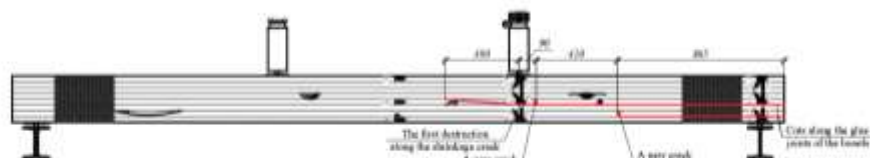
Fig. 20. General view and scheme of the experimental specimen after the first signs of strength loss
